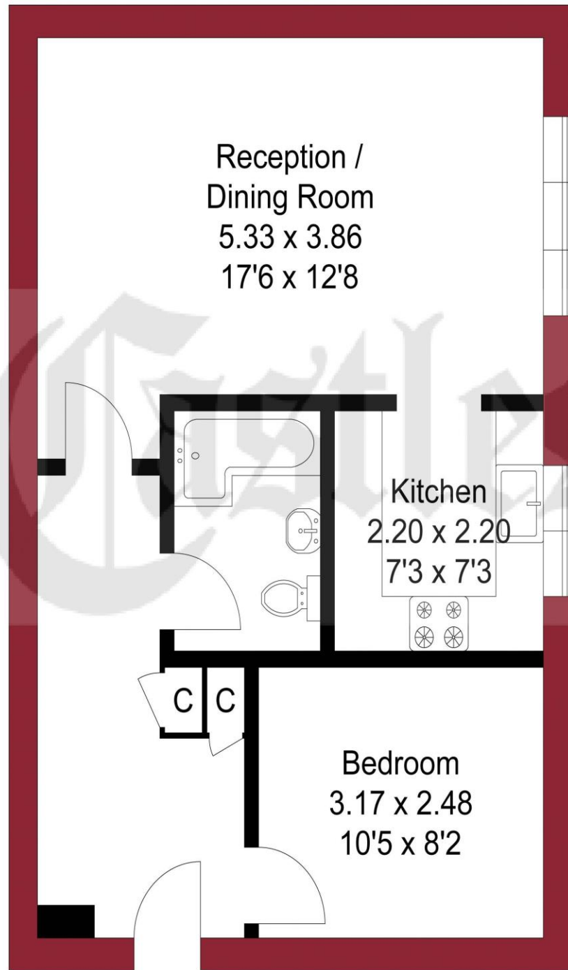
SECOND FLOOR
