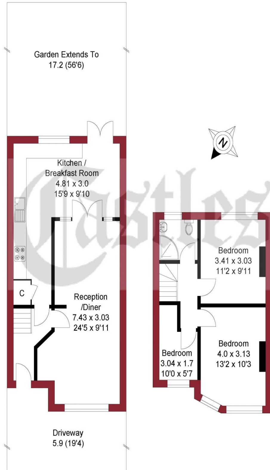
GROUND FLOOR
