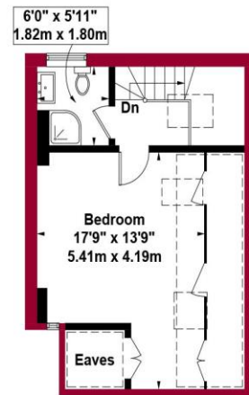
Second Floor Floor Area 400 sq ft / 37.2 sq m
