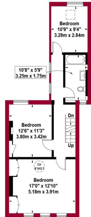
Second Floor Floor Area 400 sq ft / 37.2 sq m
