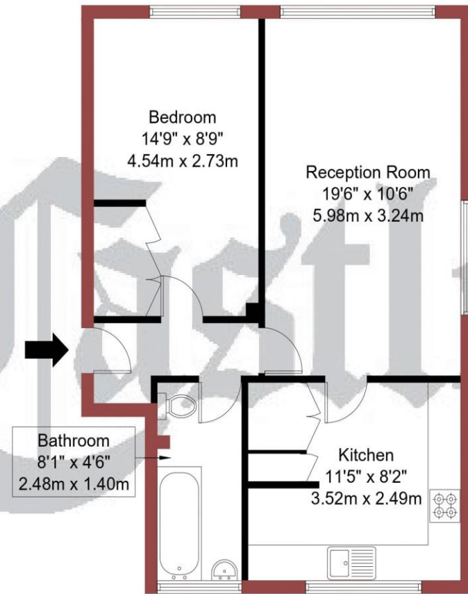
Second Floor Gross Internal Floor Area 49.2 sq m / 530 sq ft
